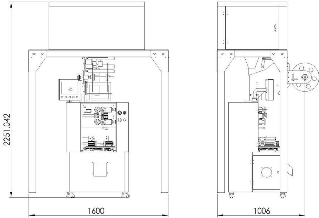
STB-50 Pyramid Tea Bag Packing Machine Drawing
