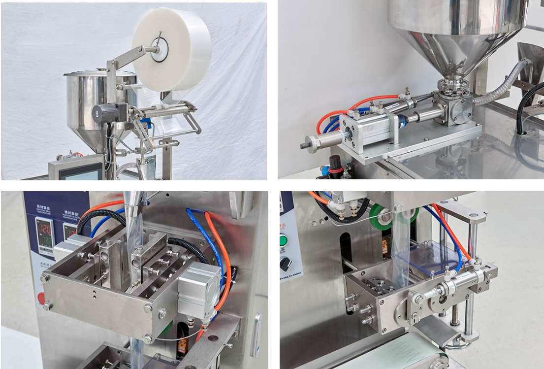
Details of Ketchup Sachet Packing Machine
