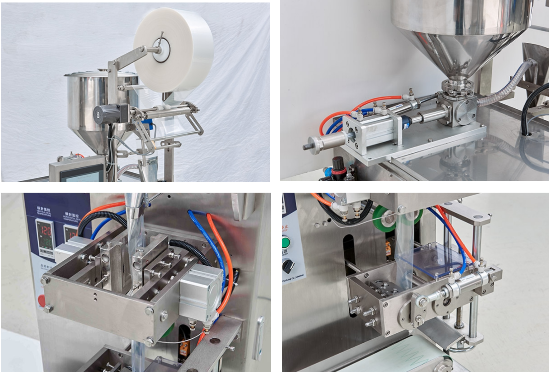
Details of Honey Sachet Packing Machine
