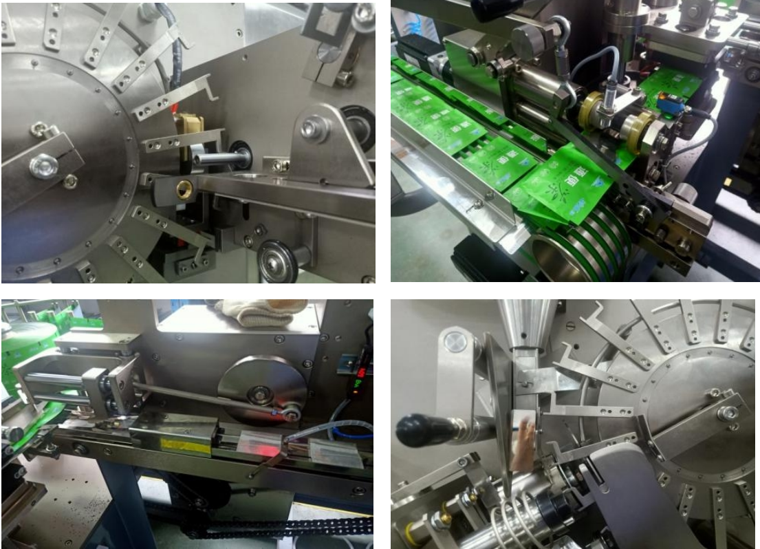
High-Speed Tea Bag Packing Machine-STB6C Details
