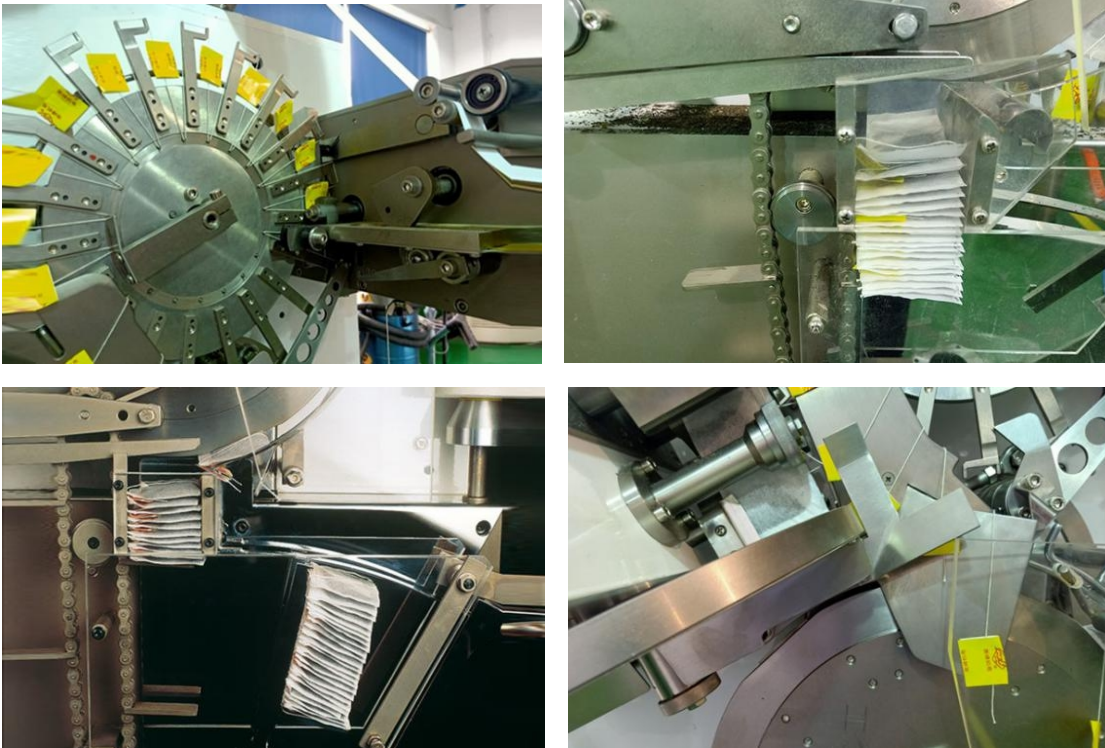
High-Speed Tea Bag Packing Machine STB-15 (With Out Package) Details
